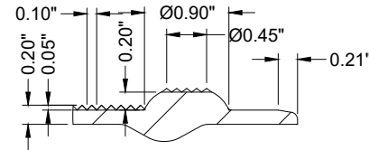
DETAIL C
